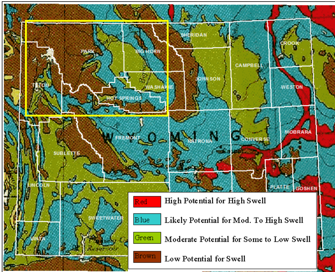
Figure 4.19. Expansive Soil Potential in Wyoming
