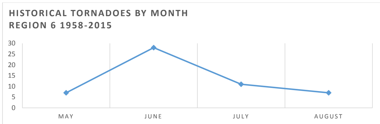
Figure 4.40. Historical Tornadoes by Month: 1958-2015
