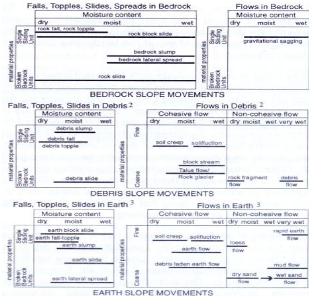
Figure 4.32. Wyoming Landslide Classifications
