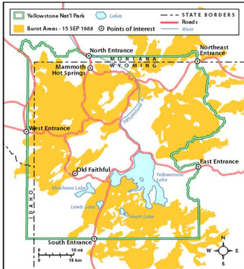
Figure 4.46. Extent of burn 1988 Yellowstone Fire
