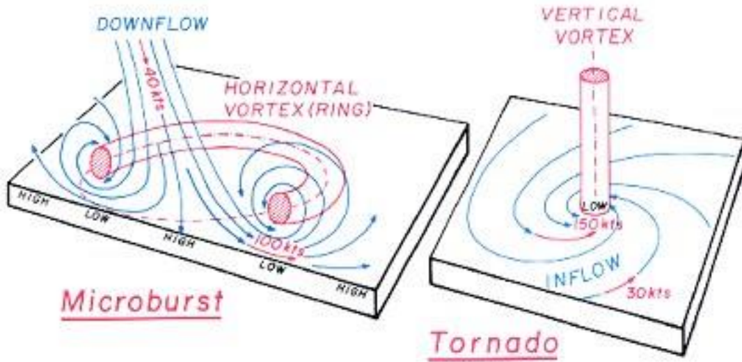
Figure 4.28. Schema of Microburst and Tornado
