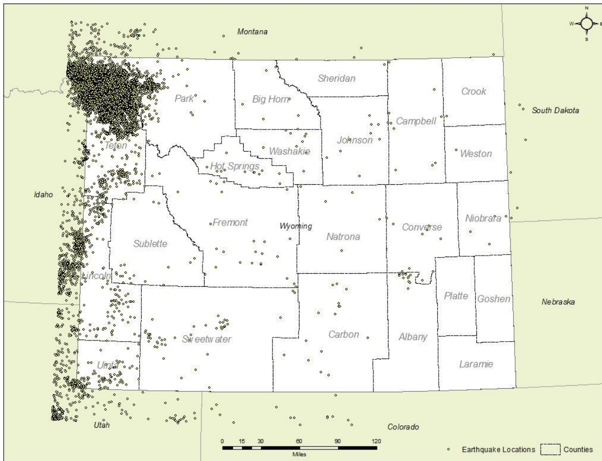
Figure 4.16. Wyoming Historic Earthquake Occurrences Statewide Since 1963- 2010
