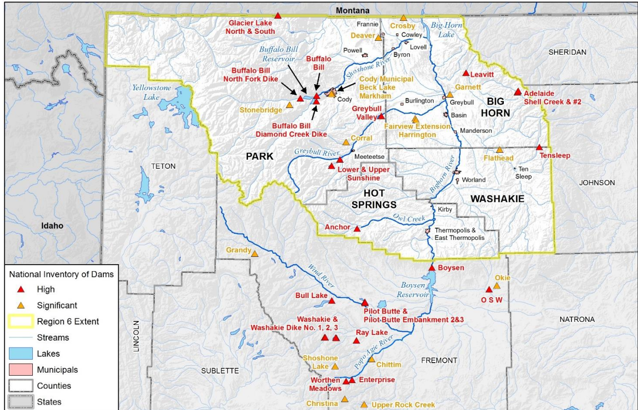
Figure 4.4. Locations of High and Significant Hazard Dams Affecting Region 6
