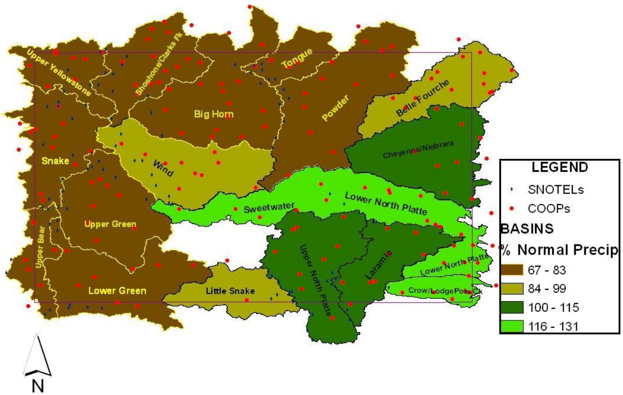
Figure 4.5. Percent of Normal Precipitation by Basin: October 2009-March 2010
