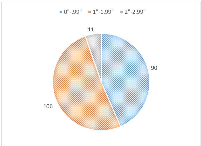
Figure 4.24. Hail Incidents by Hail Diameter Region 6 1955-2015
