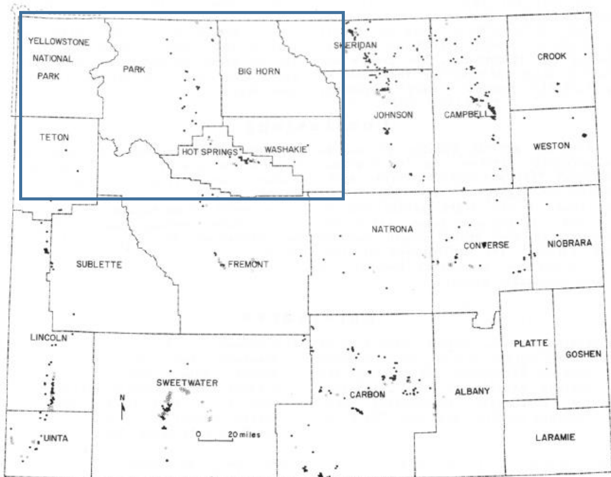
Figure 4.36. Mine Subsidence in Wyoming
