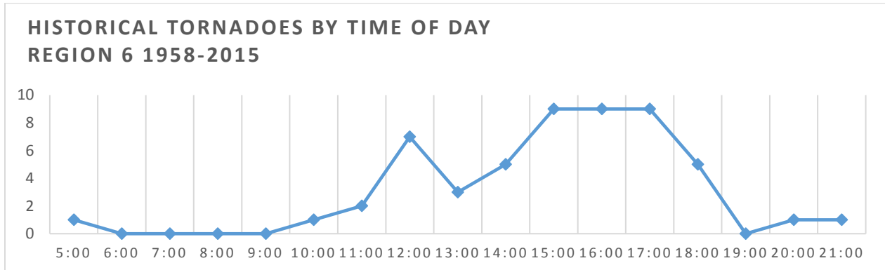
Figure 4.41. Historical Tornadoes by Time of Day: 1958-2015
