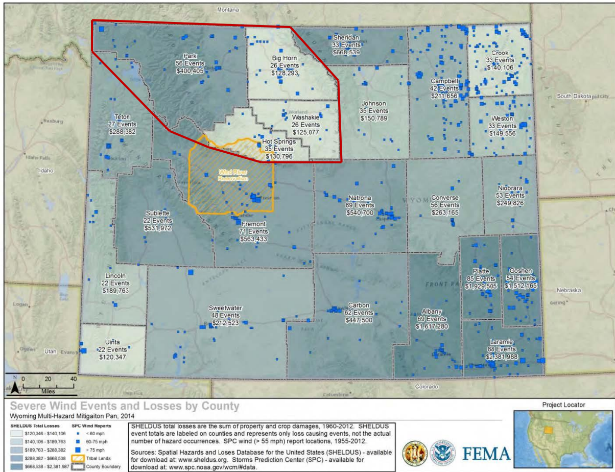
Figure 4.31. Wind Events and Losses, Wyoming 1960-2012 / Region 6 Outlined in Red
