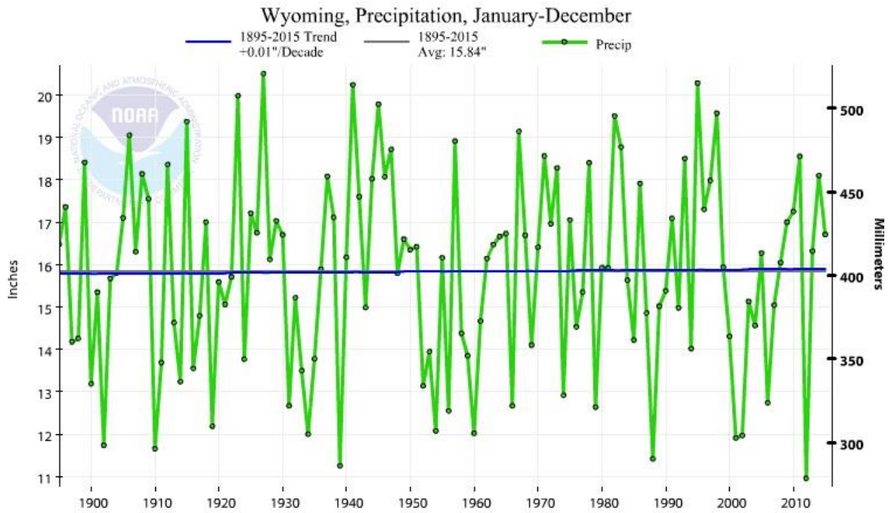
Figure 4.6. Wyoming Annual Precipitation: 1895-2015
