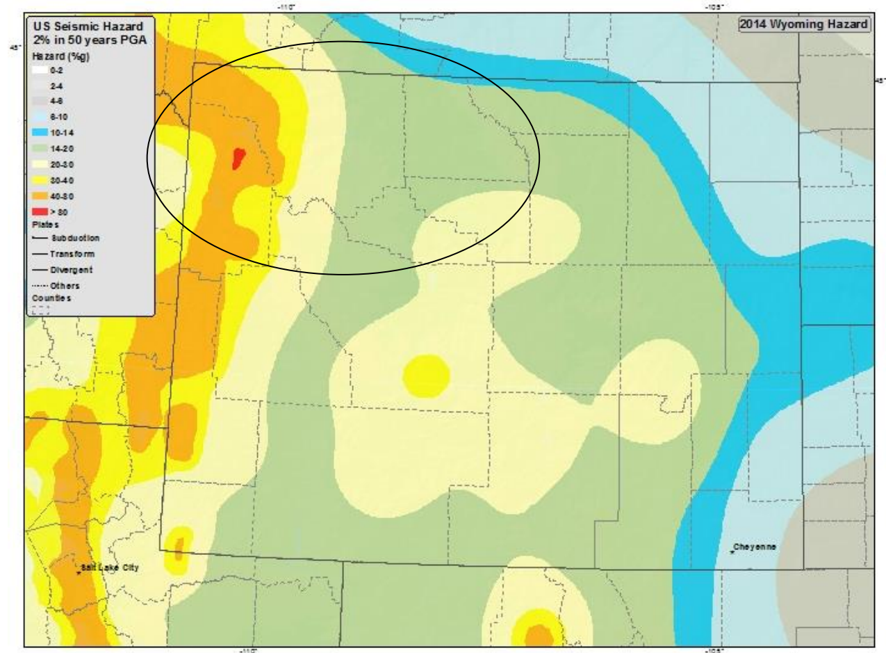
Figure 4.17. 2500-year probabilistic acceleration map (2% probability of exceedance in 50 years) – Region 6 in oval
