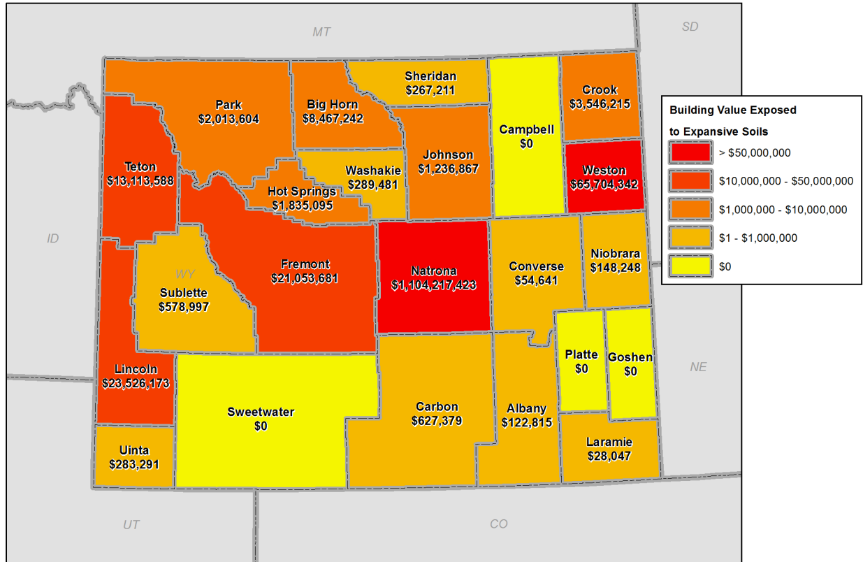
Figure 4.21. Wyoming Exposure to Shrinking/Swelling Soils by County
