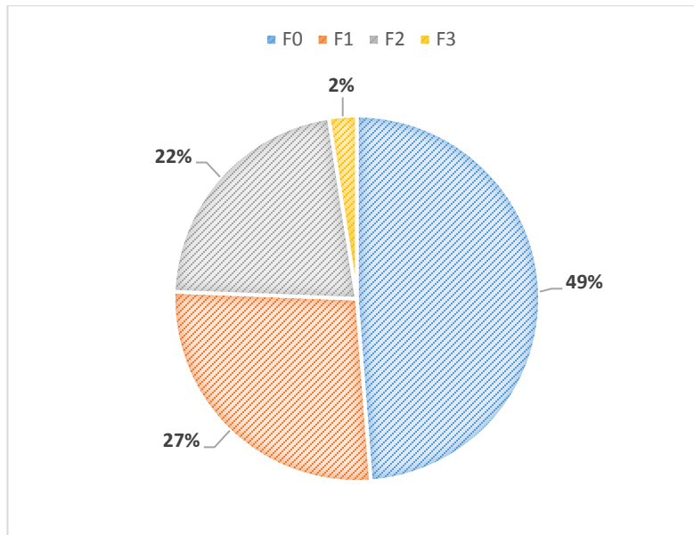
Figure 4.38. F-Scale Tornadoes by Rating
