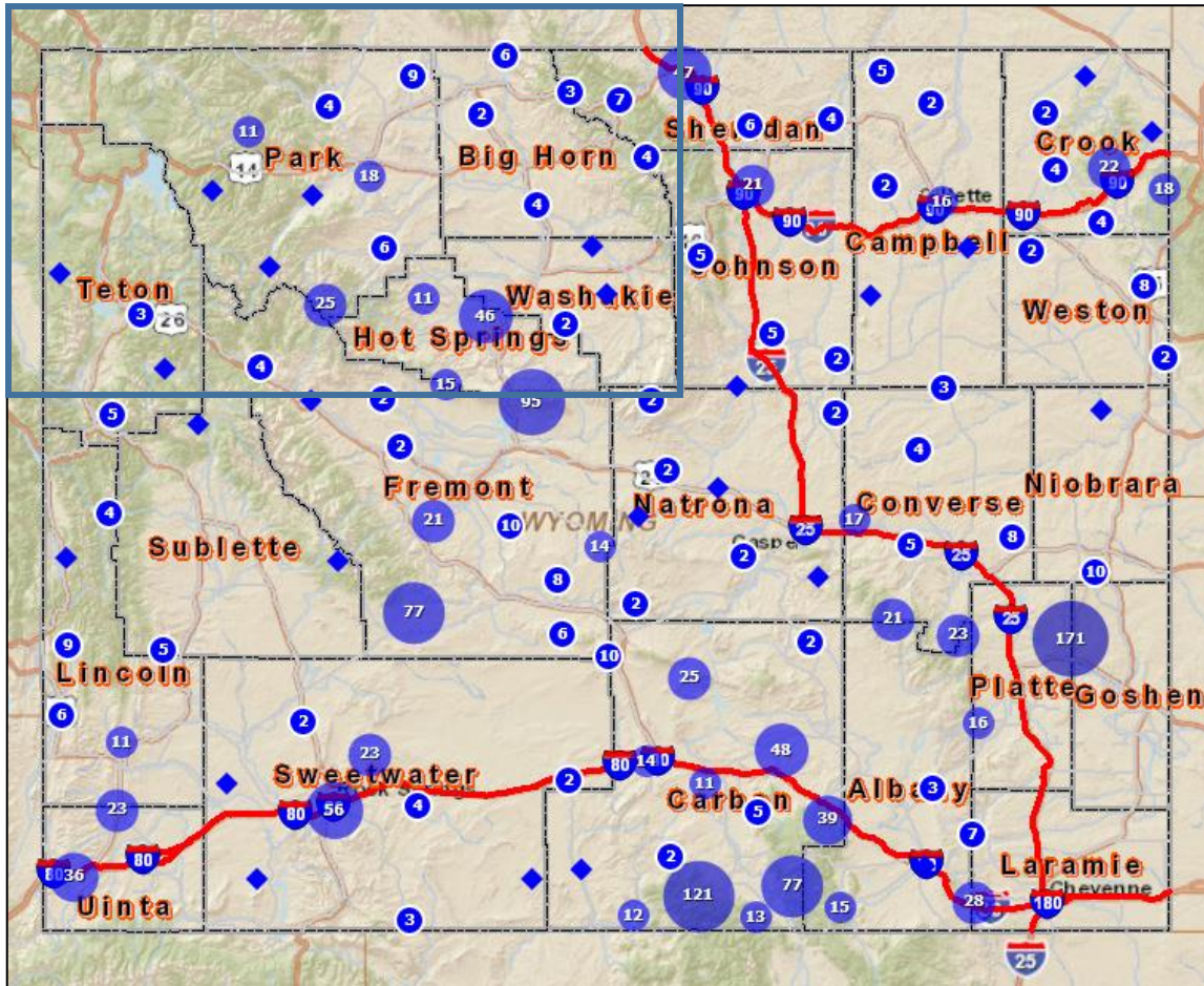
Figure 4.37. Abandoned Mine Sites with Subsidence-Prone Underground Workings
