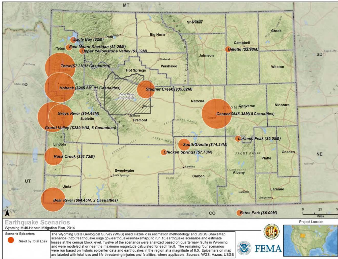
Figure 4.18. HAZUS-MH Earthquake Scenarios for Wyoming, 2011
