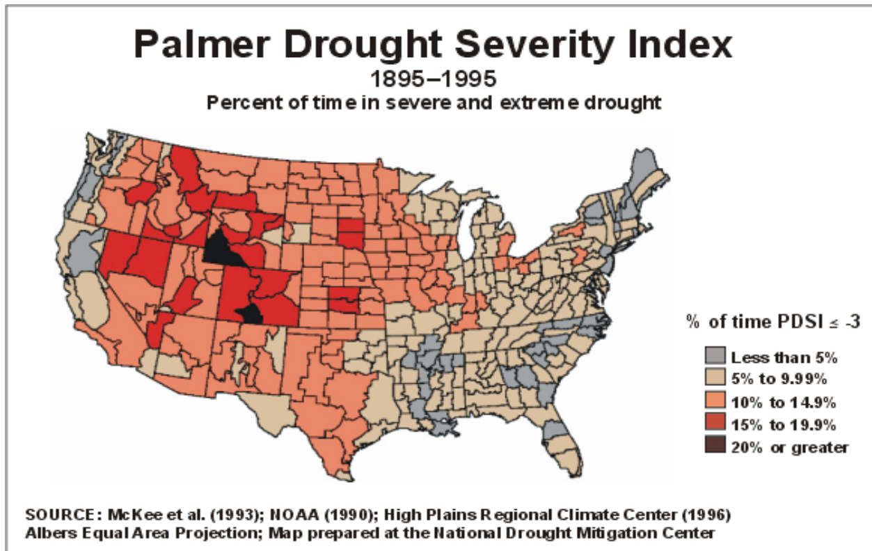
Figure 4.13. Palmer Drought Severity Index for the Continental U.S.: 1895-1995
