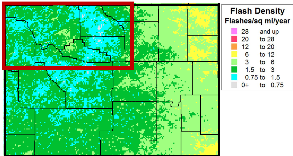
Figure 4.35. Average annual lightning flash density (flashes/sq. mi./year) 2005-2014 over Wyoming.
