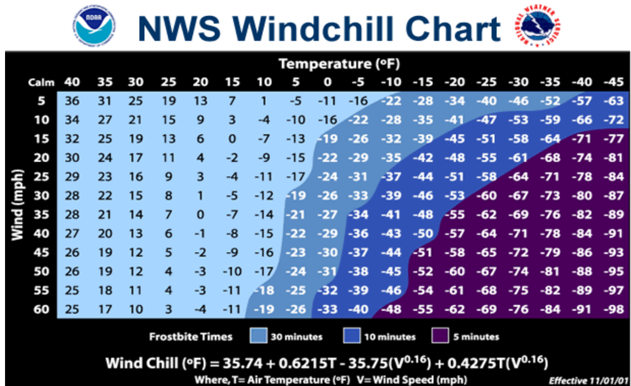
Figure 4.22. National Weather Service Wind-Chill Chart
