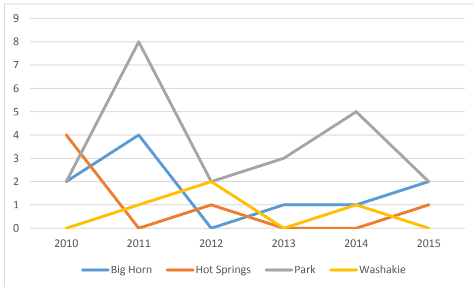
Figure 4.27. Hazardous Materials Spills/ Accidents Reported to the NRC Region 6: 2010-2015
