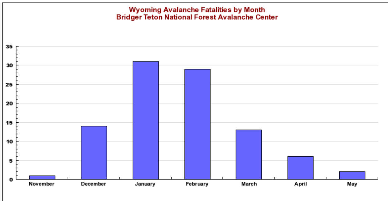
Figure 4.2. Wyoming Avalanche Fatalities by Month: 1913-2016
